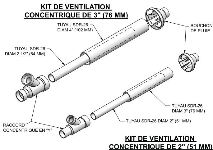
Figure 4-7 Contenu du kit
