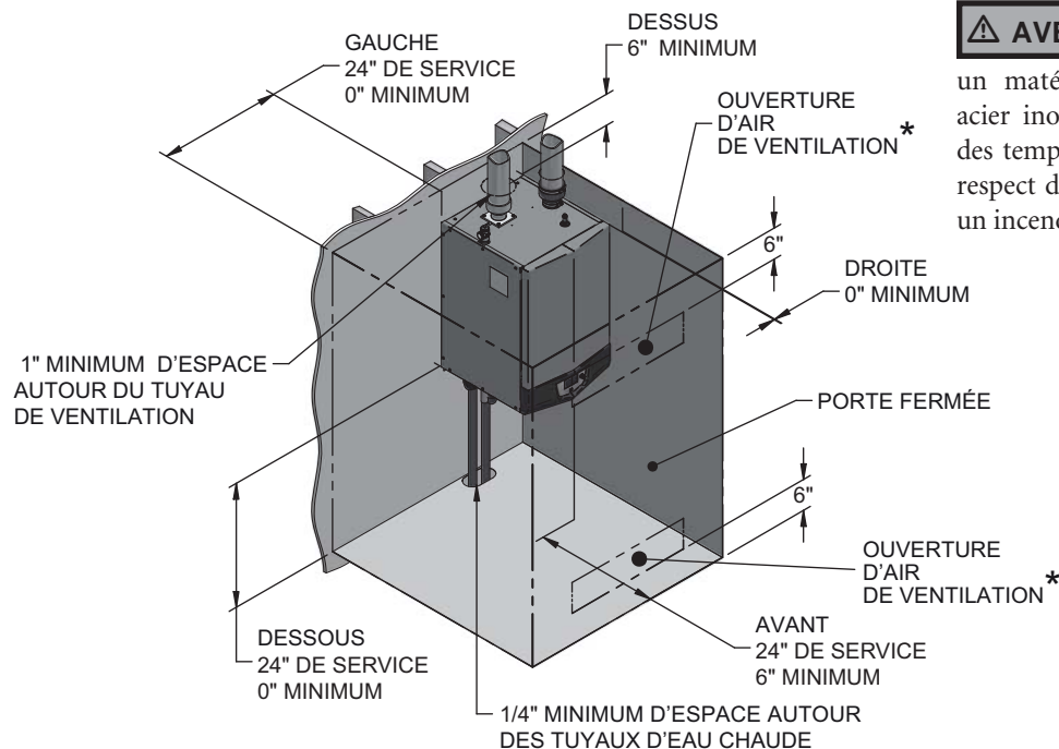
Figure 1-1 Installation en placard – Espaces minimum requis
