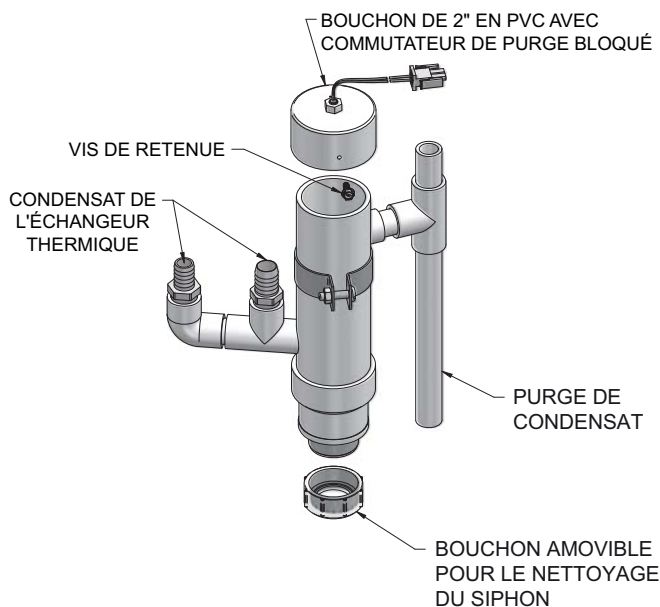
Figure 10-1 Siphon du condensat
