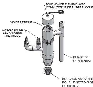
Figure 12-1 Siphon du condensat
