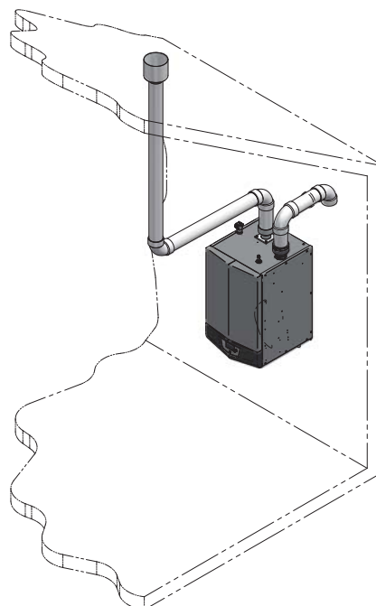
Figure 3-5 Ventilation verticale, Air latéral
